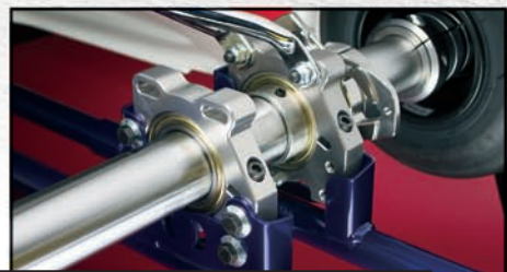
ARROW'S FULL-HEIGHT ONE-PIECE MACHINED BILLET ALLOY BEARING FLANGES
